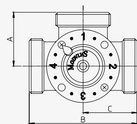
Art. 1056 - Male thread
