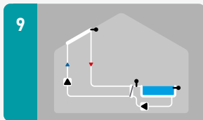
9 Solar + heat exchanger (sensor on secondary) + swimming pool
