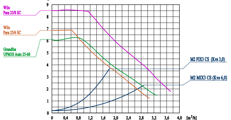
Performance curves of the pump unit and of the circulating pumps
