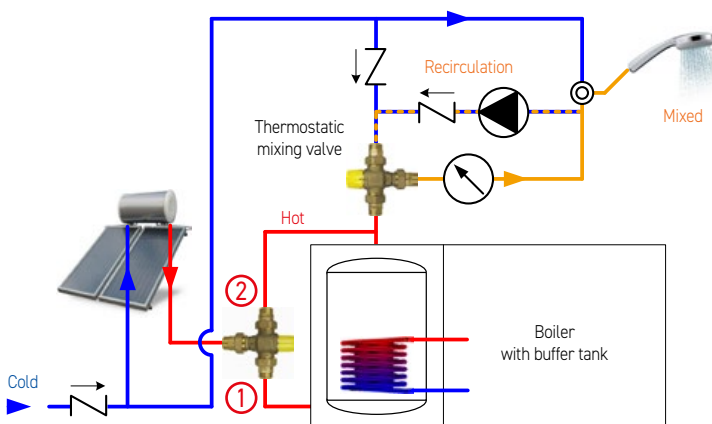
The hydraulic scheme is to be considered just an indication
